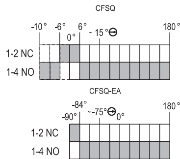
Positive opening
